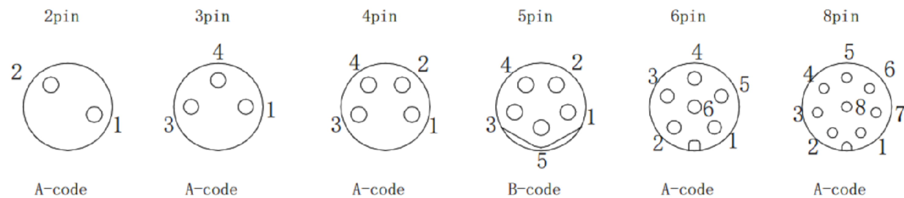
Pin assignment front view/针位分布前视图
